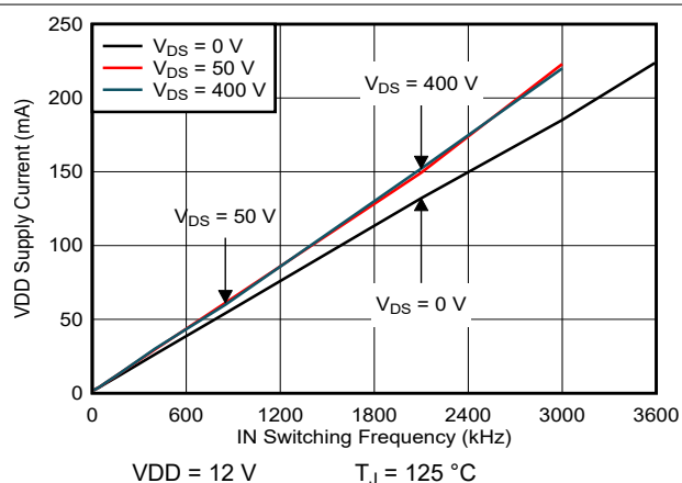
Figure 6-10. VDD Supply Current vs IN Switching Frequency
