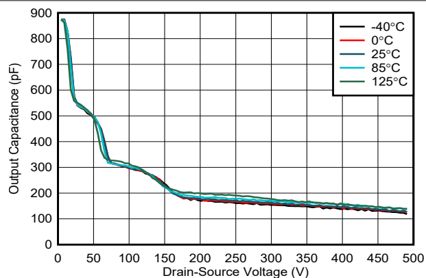
Figure 6-8. Output Capacitance vs Drain-Source Voltage
